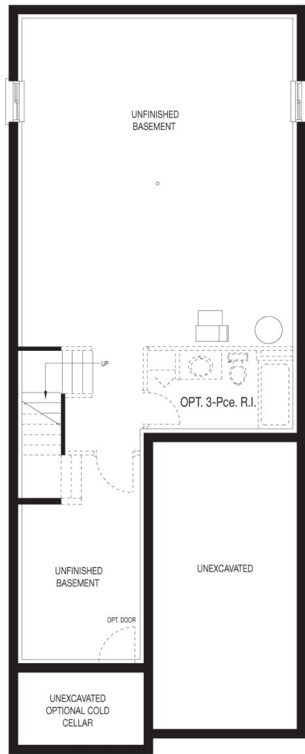
BASEMENT PLAN
